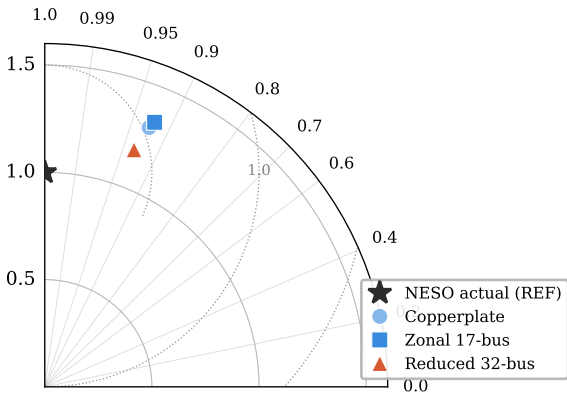
Taylor diagram — 2023 hourly CI
